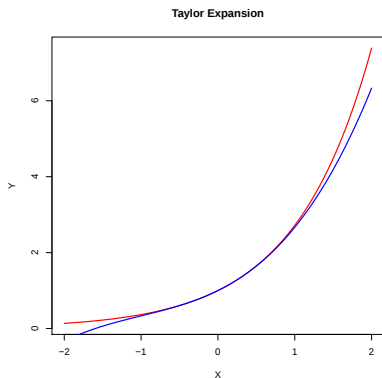
Figure : The exponential function, g(x) = e^x , and the Taylor Series approximation: x_0 = 0 , g_3(x_1) = 1 + x_1 + \frac{x^2}{2} + \frac{x^3}{6} (from Wikipedia)
