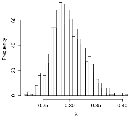
Histogram of \lambda for n = 100
